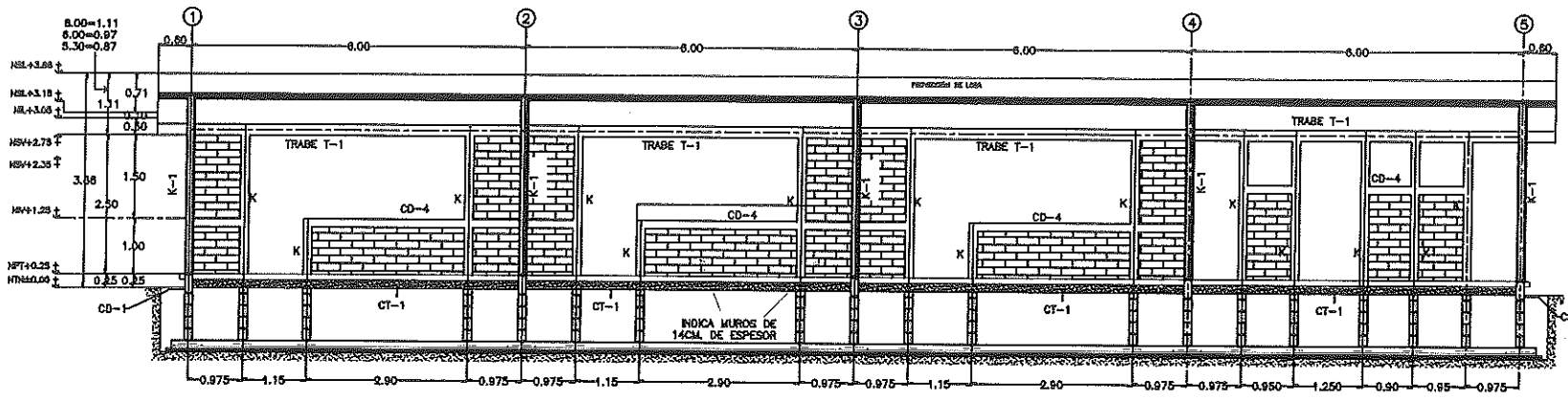
FACHADA ESTRUCTURAL PRINCIPAL
