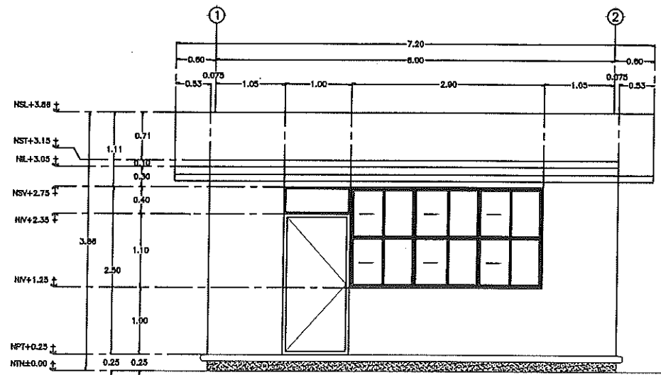
FACHADA PRINCIPAL
