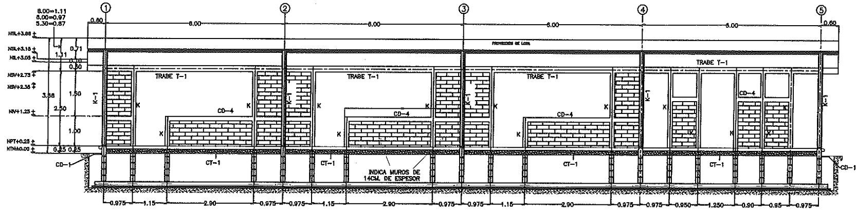
FACHADA ESTRUCTURAL PRINCIPAL
