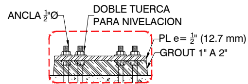
DETALLE DE-01 PLACA e=1/2" (12.7 mm)
