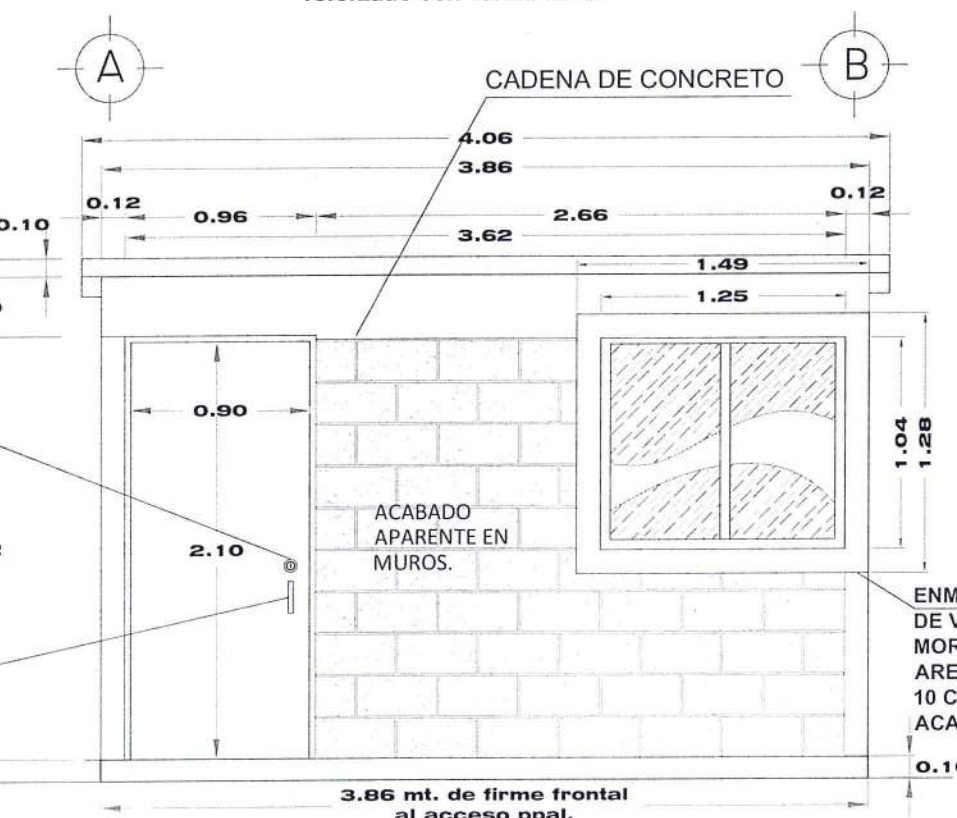
FACHADA PRINCIPAL
