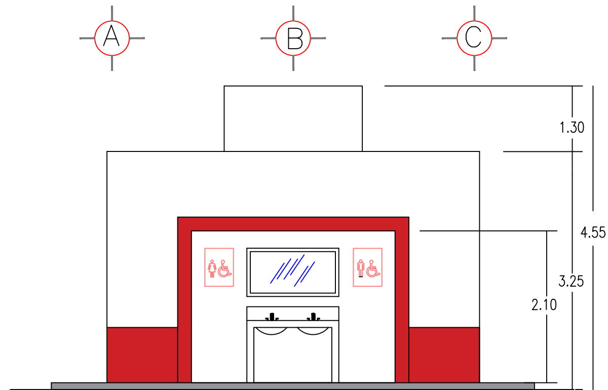
FACHADA PRINCIPAL
